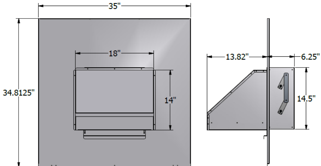
Motorized Damper
