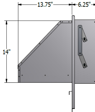
Motorized Damper
